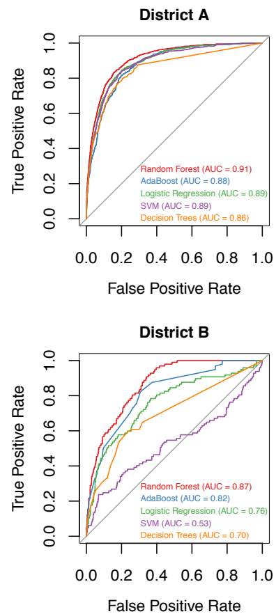
Figure 2: ROC Curves
